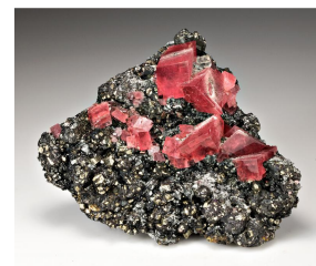
Rhodochrosite - Colorado
